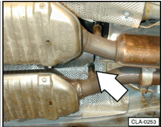
Z29 Heater for Lambda-probe 1 (2.8 ltr. engine)
