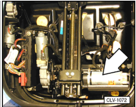
V28 Driver's seat fore/aft adjusting motor
