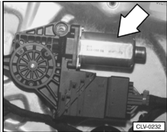
V147 Motor for window regulator, driver's side
