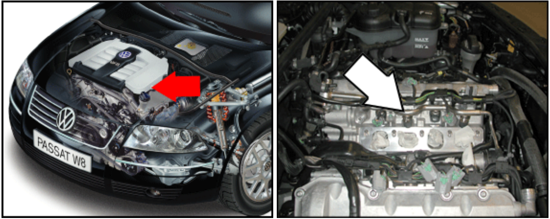
N85 Cylinder 7 Fuel Injector (4.0 ltr. engine)
