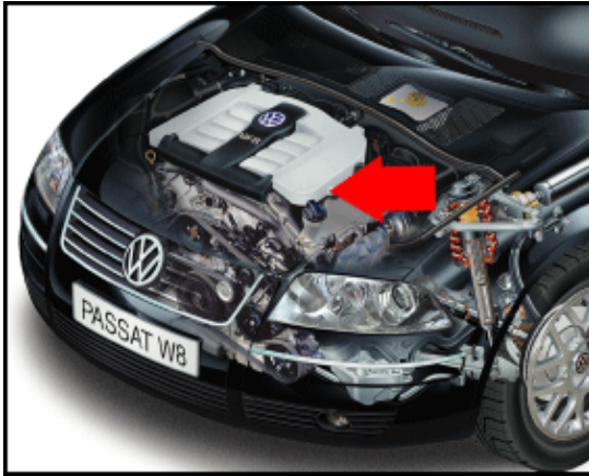
N84 Cylinder 6 Fuel Injector (4.0 ltr. engine)
