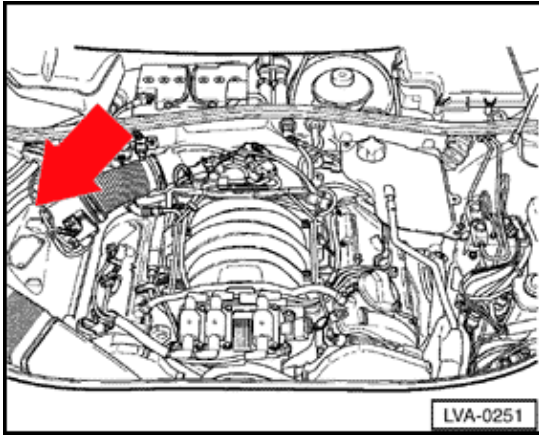
N80 Evaporative Emission (EVAP) canister purge regulator valve (2.8 ltr. engine)
