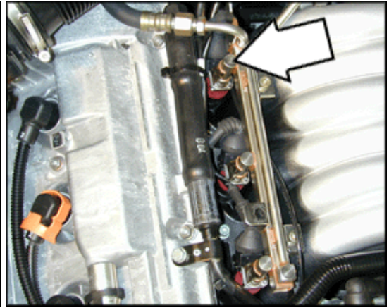
N32 Cylinder 3 Fuel Injector (2.8 ltr. engine)
