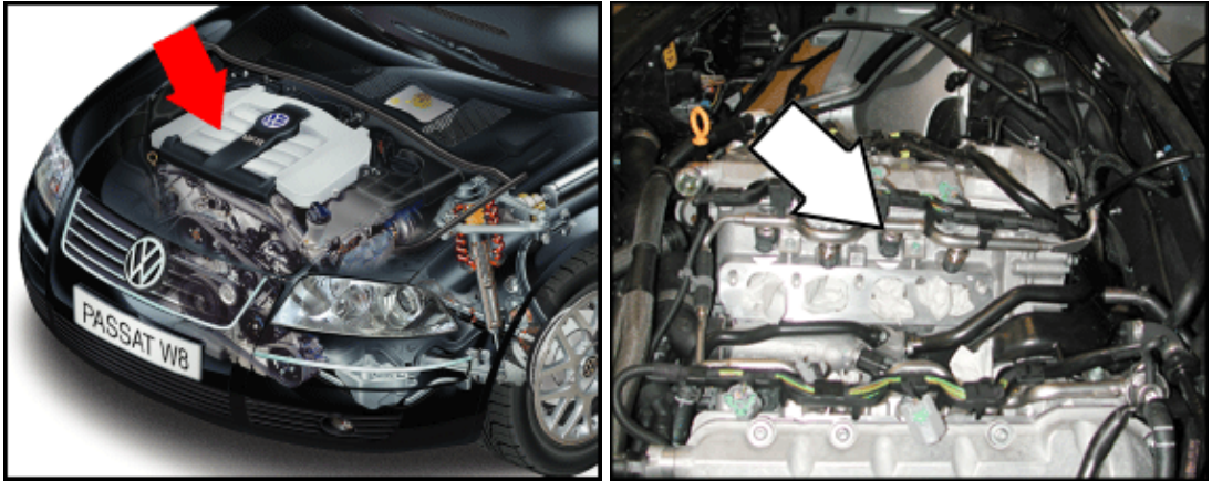
N32 Cylinder 3 Fuel Injector (4.0 ltr. engine)
