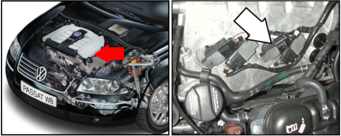
N325 Ignition Coil 7 with Power Output Stage (4.0 ltr. engine)
