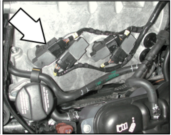
N323 Ignition Coil 5 with Power Output Stage (4.0 ltr. engine)
