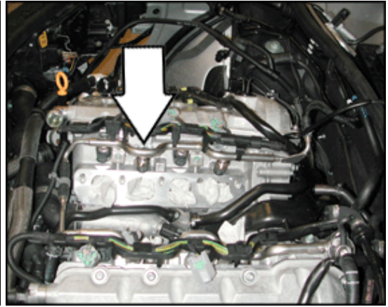
N31 Cylinder 2 Fuel Injector (4.0 ltr. engine)
