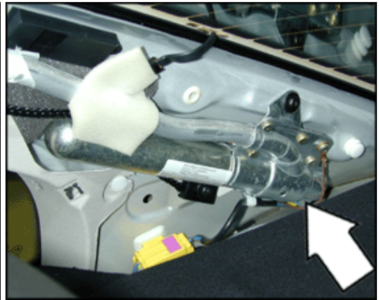
N252 Front Passenger Head Airbag Igniter
