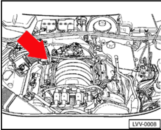
N205 Valve 1 for camshaft adjustment (2.8 ltr. engine)
