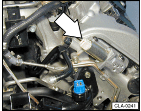
N205 Valve 1 for camshaft adjustment (2.8 ltr. engine)
