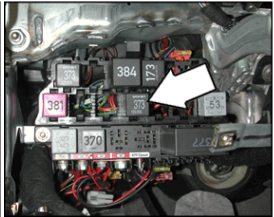
J569 Brake Booster Relay (gasoline engines)
