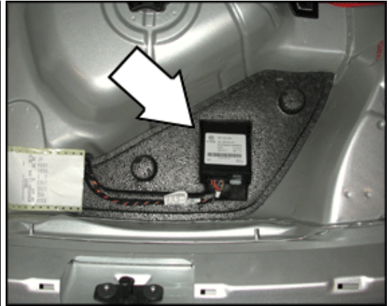
J538 Fuel Pump (FP) Control Module (4.0 ltr. engine)
