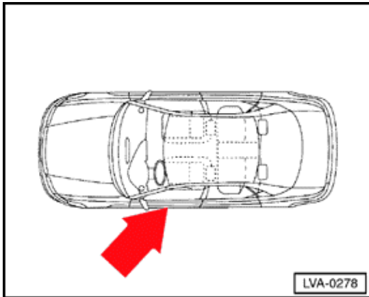
J386 Door control module, driver's side
