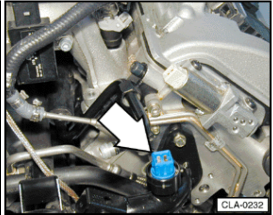
G62 Engine Coolant Temperature (ECT) sensor (2.8 ltr. engine)
