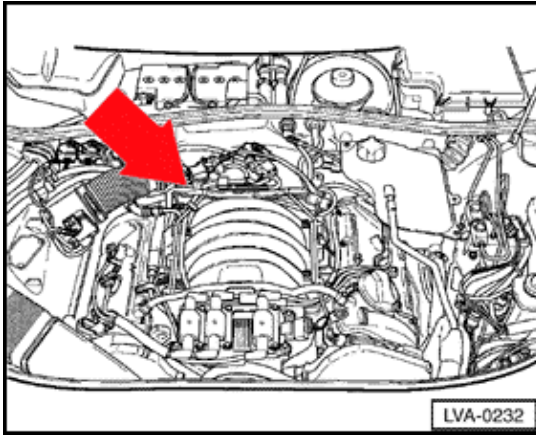
G62 Engine Coolant Temperature (ECT) sensor (2.8 ltr. engine)
