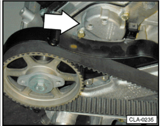
G40 Camshaft Position (CMP) sensor (2.8 ltr. engine)
