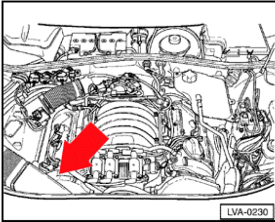
G40 Camshaft Position (CMP) sensor (2.8 ltr. engine)
