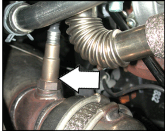
G39 Heated Oxygen Sensor (HO2S) (2.0 ltr. tdi engine)
