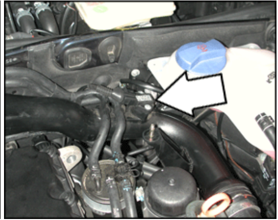
G31 Charge Air Pressure Sensor (2.0 ltr. tdi engine)
