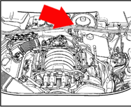
G294 Brake Booster Pressure Sensor (gasoline engines)
