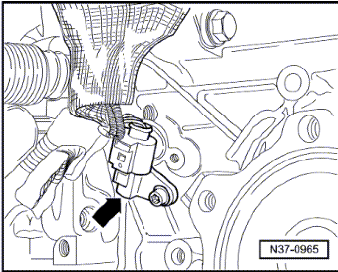
G28 - Engine Speed (RPM) Sensor
