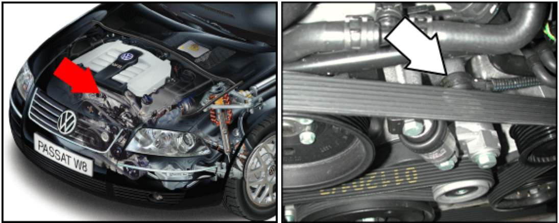
G198 Knock sensor 3 (4.0 ltr. engine)
