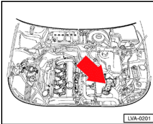
G187 Angle sensor –1– for throttle drive (power accelerator actuation) (1.8 ltr. engine)
