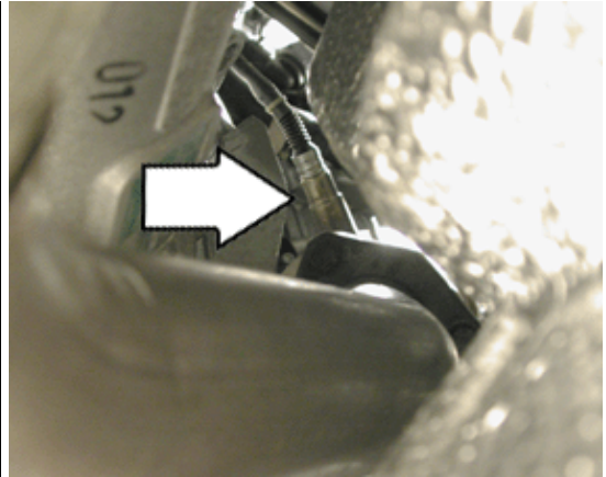
G130 Oxygen Sensor (O2S) Behind Three Way Catalytic Converter (TWC) (4.0 ltr. engine)
