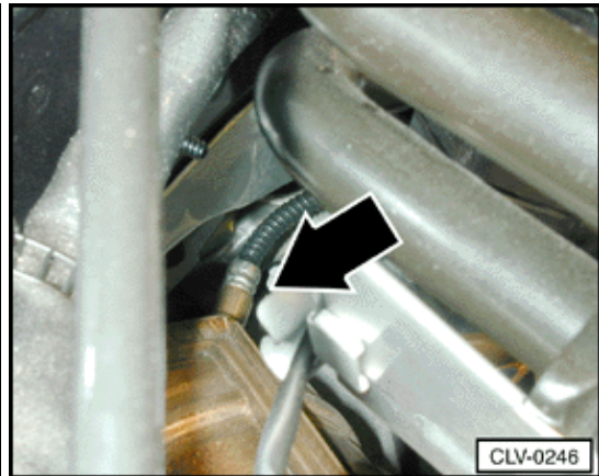
G130 Oxygen sensor behind Three Way Catalytic Converter (TWC) (1.8 ltr. engine)
