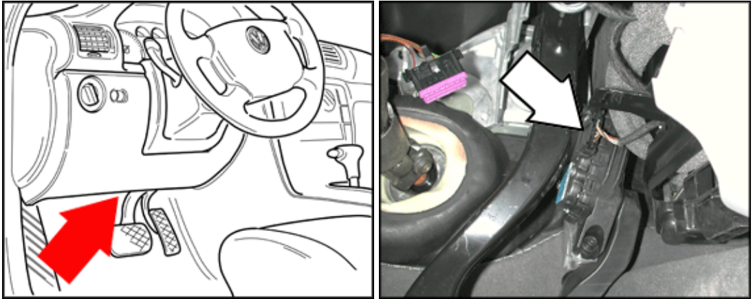
F60 Closed Throttle Position (CTP) Switch (2.0 ltr. tdi engine)
